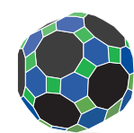
Truncated Icosidodecahedron
