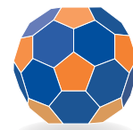
Truncated Icosahedron
